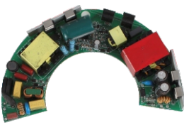
200W认证开关电源 200W certified switching power supply
