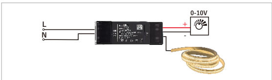
0-10V调光【连接示意图】 0-10V Dimmer Connection diagram
