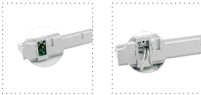
两种接线方式可选 Two Wiring options are available 单位/UNIT: mm
